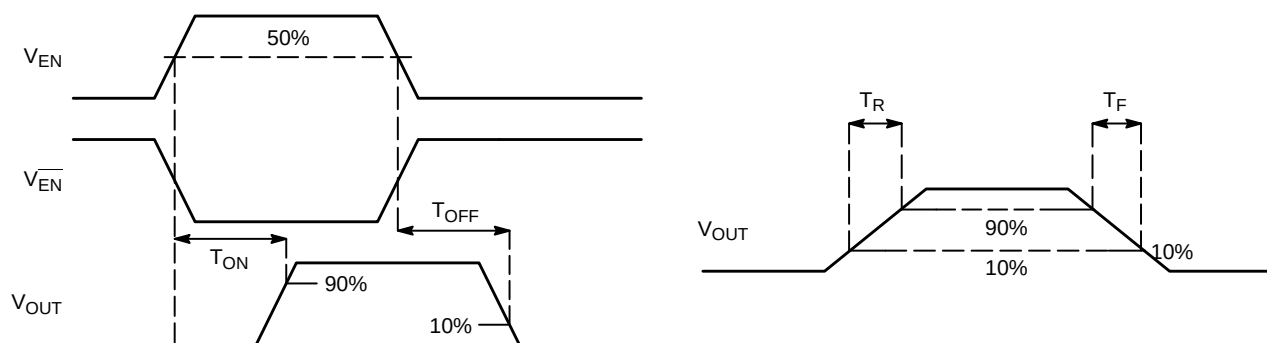
Figure 4. Voltage Waveform
